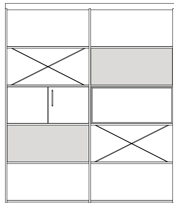
front view / vista frontal L1600 -1656 x 367 x1940
